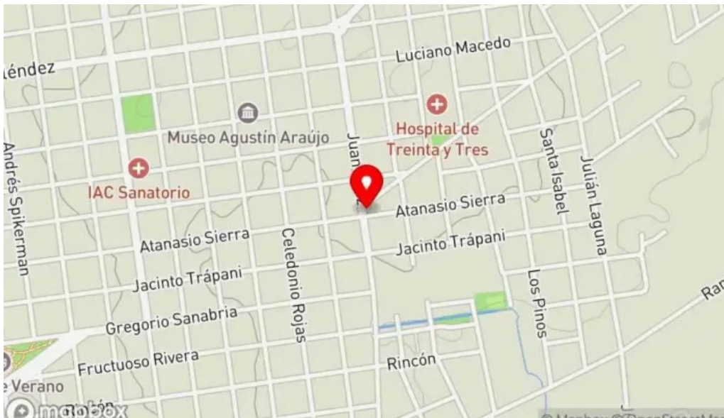
Karma map
